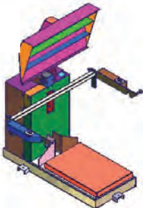
control elements RC 1100 TT
